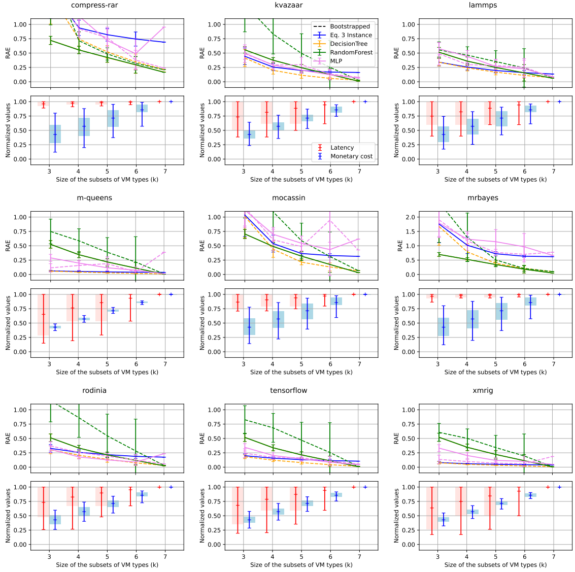
Fig. 3. Results with the C7i family for all benchmark applications
